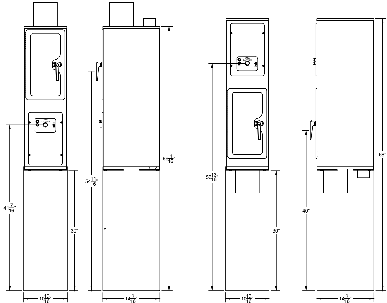
HT15-6" DOWN SEND UNIT MOUNTED ON PEDESTAL
